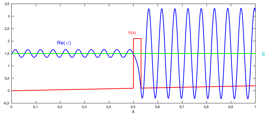
Fig. 8. Tunnelling structure with injection of a plane wave from the right ( x = 1 ). Red curve: piecewise linear potential V(x) with applied bias. Blue curve: \Re(\psi(x)) , real part of the wave function that is partly transmitted, but mainly reflected in this example; \varepsilon = 0.01 . Green line: energy of the injected plane wave with E < \max V(x) .
