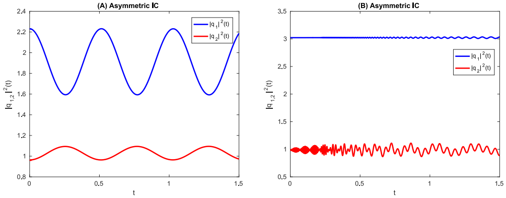
Fig. 21. The asym.lin.case. Left: Evolution in time of the numerical solutions |q_1|^2(t) resp. |q_2|^2(t) with the set of parameters (A). Right: Same plots with the set of parameters (B).
