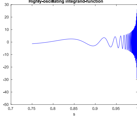
Fig. 19. Evolution in time of the integrand function h(s) := \frac{1}{\sqrt{1-s}} e^{i\frac{a^2}{1-s}} with s \in [0, 1] .
