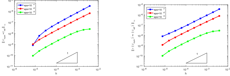
Fig. 10. Absolute error (in the L^\infty -norm and log-log scale) between the computed solution and a reference solution (obtained with h = 2^{-18} \approx 4 \cdot 10^{-6} ), for a piecewise linear potential. Left: \|\psi_{ref} - \psi_{num}\|_\infty . Right: \|\epsilon(\psi_{ref}) - \epsilon(\psi_{num})\|_\infty .
