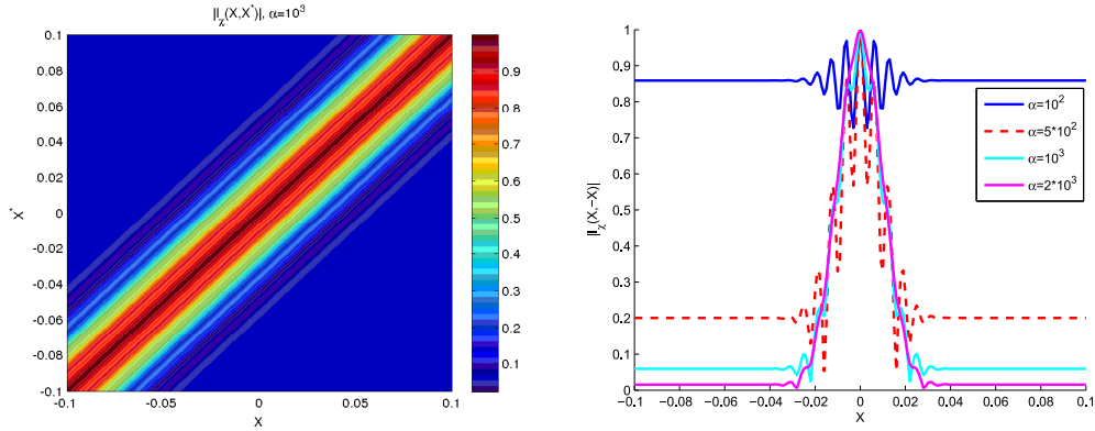
Fig. 14. Left: Plot of |I_\chi(X, X')| for \alpha = 10^3 . Right: Plot of |I_\chi(X, -X)| for several values of \alpha .
