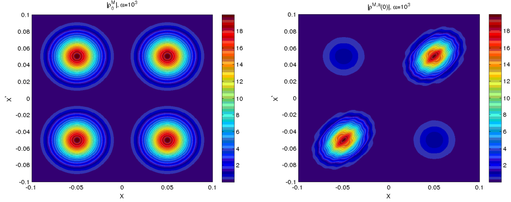
Fig. 13. Test case: Dirac potential with \alpha = 10^3 . Left: Plot of |\rho_0^M(X, X')| before the collision; Right: Plot of |\rho^{M,a}(0, X, X')| immediately after the collision.
