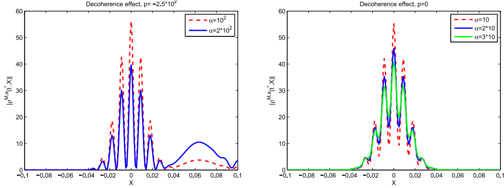
Fig. 16. Attenuation of the interference pattern of the heavy particle, in the case that the light particle comes from the right with p = -2.5 * 10^2 (left Fig.) resp. p = 0 (right Fig.).
