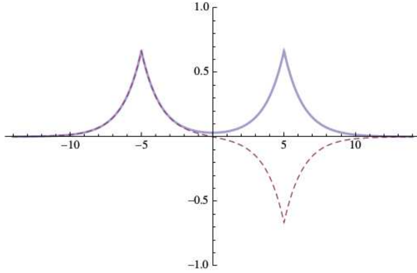
Fig. 18. Plot of the functions \phi_f(x) in blue and \phi_e(x) with a dashed line.
