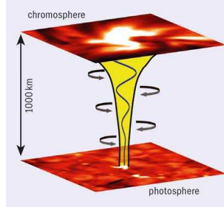
Fig. 3. Creation of an Alfvén wave, propagating between two levels of the solar atmosphere.
