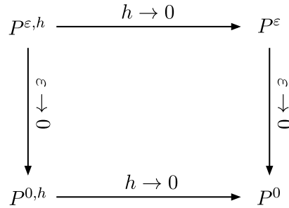
Fig. 7. Properties of AP-schemes.
