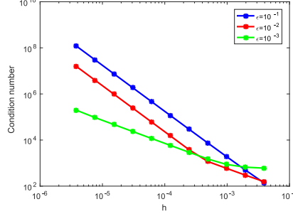
Fig. 11. Condition number for the discrete BVP in Ex. 2, as a function of h , for three values of \varepsilon .
