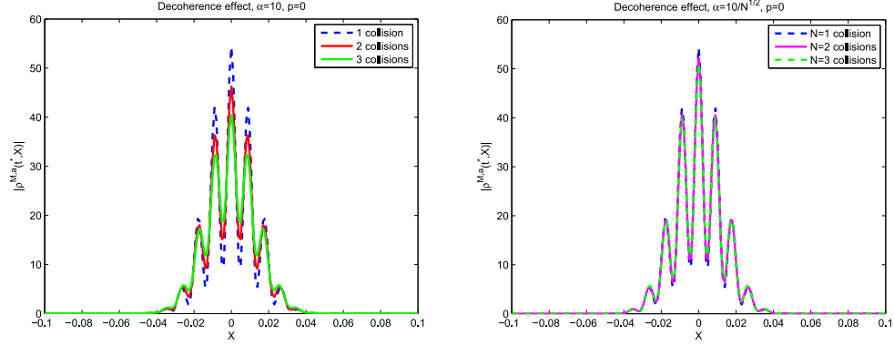
Fig. 17. Attenuation of the interference pattern of the heavy particle in the case of several collisions. Test case: Dirac's delta potential, p = 0 . Left: Fixed \alpha = 10 and several collisions N = 1, 2, 3 . Right: N = 1, 2, 3 with \alpha = 10/\sqrt{N} .
