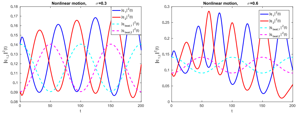
Fig. 23. The non-linear time-evolution of the numerical solutions |q_1^{num}|^2(t) resp. |q_2^{num}|^2(t) (in blue/red full line) and corresponding linear beating solutions |q_{beat,1}|^2(t) resp. |q_{beat,2}|^2(t) (in cyan/magenta dashed line), for \sigma = 0.3 (left) and \sigma = 0.6 (right).
