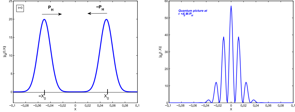
Fig. 12. Left: Probability density associated to the initial state of the heavy particle. Right: Probability density associated to the state of the heavy particle in the case of no interaction, at the time of maximal overlap of the two bumps.
