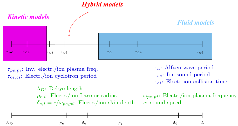
Fig. 6. Different time and space scales occurring in a fusion plasma.
