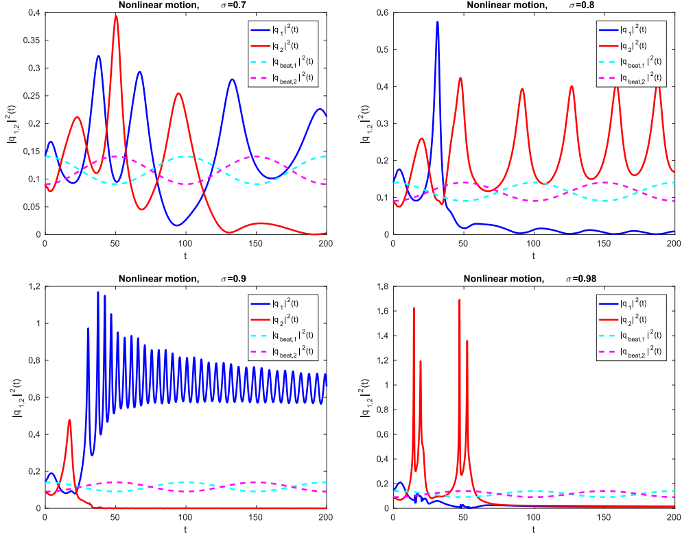
Fig. 24. The non-linear time-evolution of the numerical solutions |q_1^{num}|^2(t) resp. |q_2^{num}|^2(t) (in blue/red full line) and corresponding linear beating solutions |q_{beat,1}|^2(t) resp. |q_{beat,2}|^2(t) (in cyan/magenta dashed line), for \sigma = 0.7 , \sigma = 0.8 , \sigma = 0.9 and \sigma = 0.98 .
