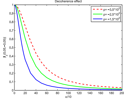
Fig. 15. The quantity |I_\chi(0.05, -0.05)| as a function of \alpha for three different values of the momentum of the light particle.
