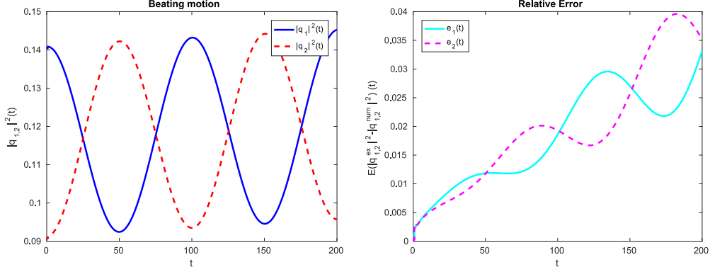
Fig. 20. The beating effect. Left: Evolution in time of the numerical solutions |q_1|^2(t) resp. |q_2|^2(t) . Right: Relative error: \text{abs}[|q_{1,2}^{ex}|^2 - |q_{1,2}^{num}|^2] / ||q_{1,2}^{ex}||_\infty .
