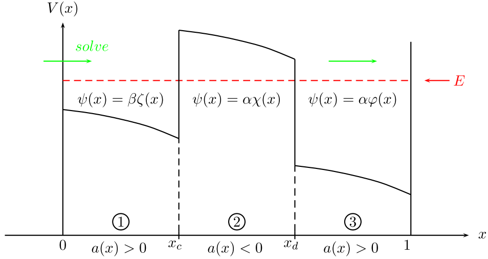
Fig. 9. Tunnelling structure: While electrons are injected from the right boundary with energy E , the decomposed problem has to be solved from left to right (as an IVP–BVP–IVP). a(x) := E - V(x) .
