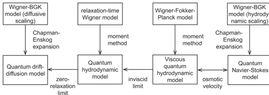
Fig. 1. Model hierarchy. The Wigner models are explained in Section 2.4.
