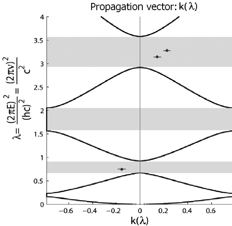
Fig. 1. The band gap structure of a photonic crystal. The band gaps are plotted in light grey while crossed dots are allowed energy levels introduced by an impurity. The axis units are arbitrary.
