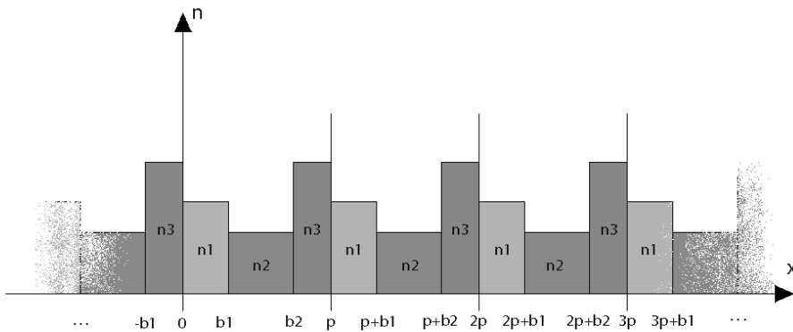
Fig. 4. Example of a periodic structure with period p in the case of a piecewise constant refractive index.
