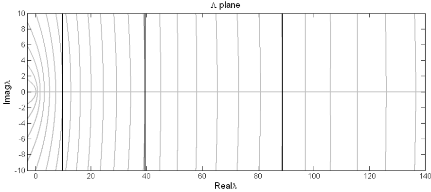
Fig. 2. \Lambda plane. The real axis and the \Gamma -curve are plotted in light grey. The vertical asymptotes, Real\{\lambda\} = (i\pi)^2 , where i = 1, 2, \dots , are plotted in black.
