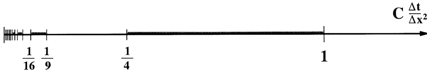
Fig. 2 - Discretized TBC of Mayfield: Stability regions.
