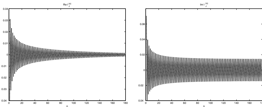
Fig. 13 - Example 2: Inverse \mathcal{Z} -transformation using ENTCAF: Numerically obtained values for Re l_j^{(n)} , Im l_j^{(n)} compared to the exact ones.
