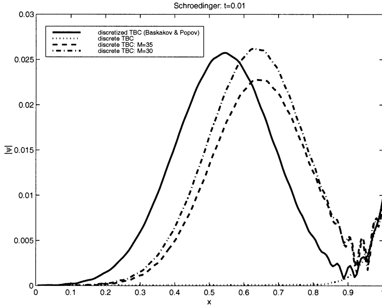
Fig. 8 - Solution |\psi(x, t)| at time t = 0.01 : the solution with the discretized TBCs of Baskakov and Popov [6] (—) in comparison to the solution using the simplified DTBC (3.85) with M = 30 (-.-.) and M = 35 (---).
