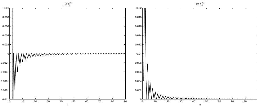
Fig. 14 - Example 2: Inverse \mathcal{Z} -transformation using ENTCAF: Numerically obtained values for \text{Re } s_j^{(n)} , \text{Im } s_j^{(n)} compared to the exact ones.
