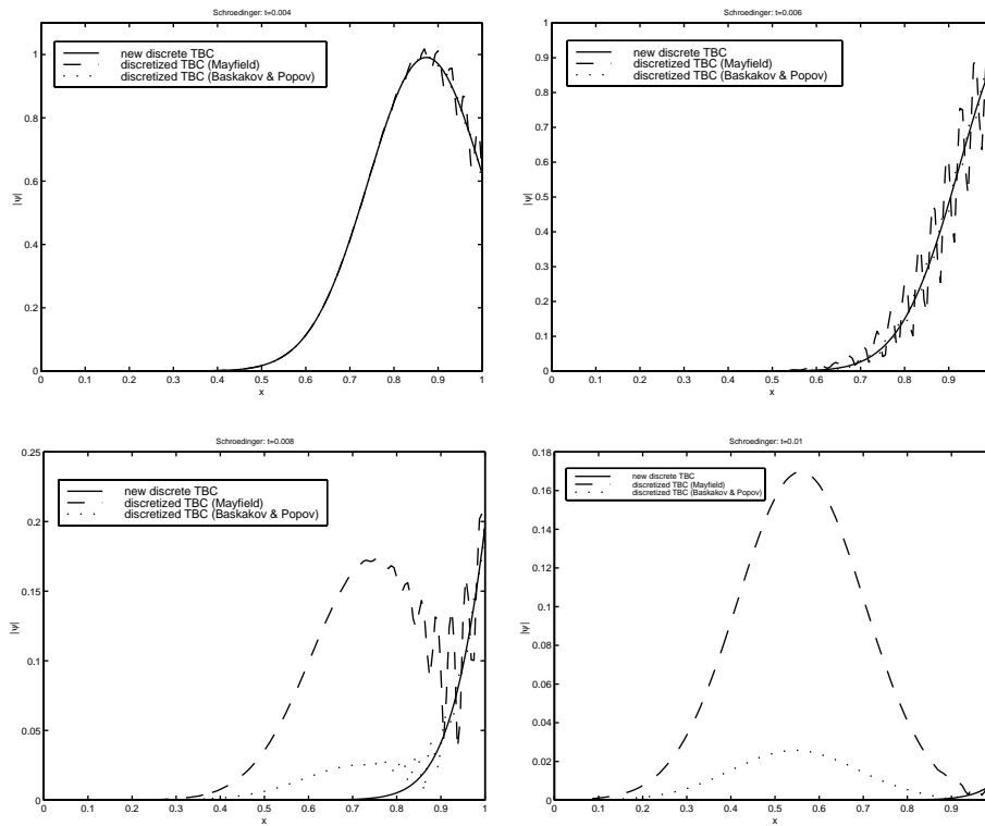
Fig. 6 - Solution |\psi(x, t)| at time t = 0.004 , t = 0.006 , t = 0.008 , t = 0.01 : the solution with the new discrete TBCs (—) coincides with the whole-space solution, while the solution with the discretized analytic TBCs (3.7) from [30] (---) or from [6] (···) introduces strong numerical reflections.
