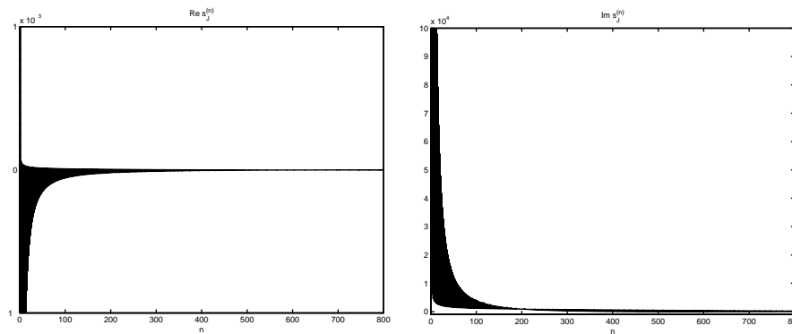
Fig. 16 - Example 3: Inverse \mathcal{Z} -transformation using ENTCAF: Numerically obtained values for \text{Re } s_j^{(n)} , \text{Im } s_j^{(n)} compared to the exact ones. In both plots only one curve is visible since the results from both approaches match so closely.
