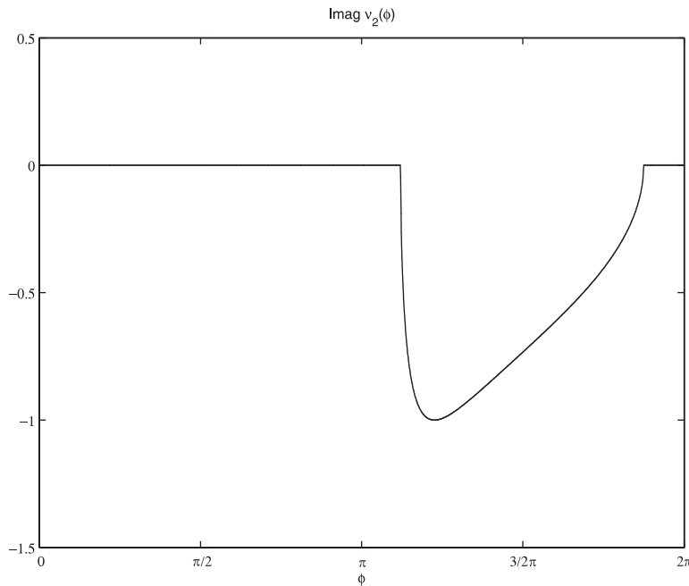
Fig. 5 - Imaginary part of \nu_2(z) on the unit circle z = e^{i\varphi} , 0 \leq \varphi \leq 2\pi .
