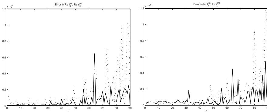
Fig. 15 - Example 2: Inverse \mathcal{Z} -transformation using ENTCAF: Difference between the numerical and exact value of the real and imaginary part of l_j^{(n)} (—) and s_j^{(n)} (⋯).
