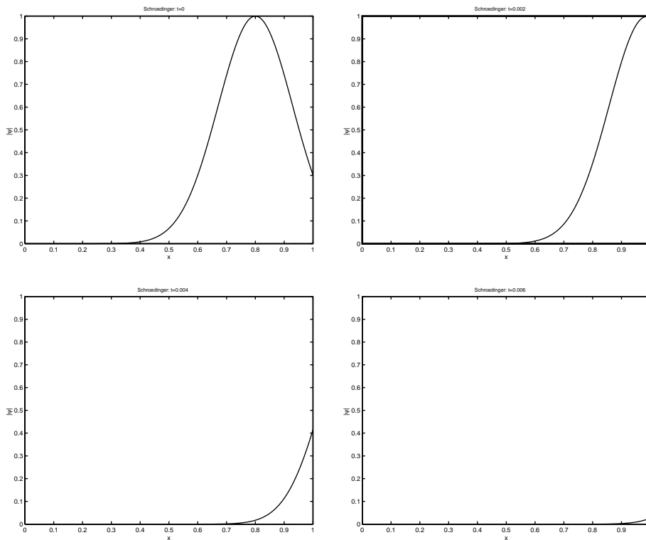
Fig. 9 - Solution |\psi(x, t)| at time t = 0, t = 0.002, t = 0.004, t = 0.006 : the solution with the new discrete TBCs (4.32) coincides with the whole-space solution and does not introduce any numerical reflections.
