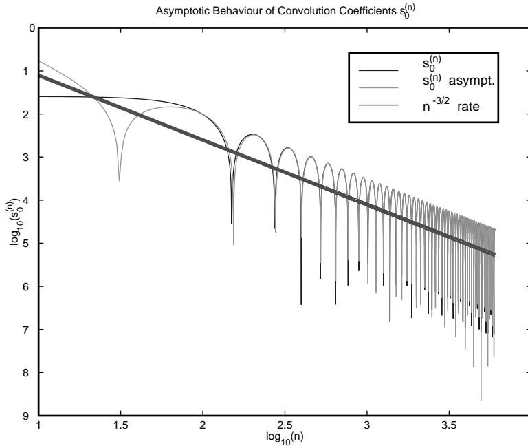
Fig. 4 - New discrete TBC: convolution coefficients s_0^{(n)} compared to the r.h.s. of (3.62) and the decaying rate (3.69).
