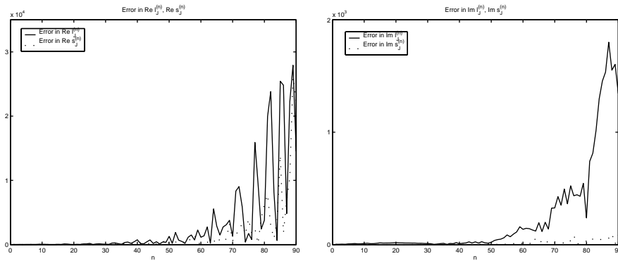
Fig. 12 - Example 1: Difference between the numerical and exact value for of the real and imaginary part of l_j^{(n)} (—) and s_j^{(n)} (···).
