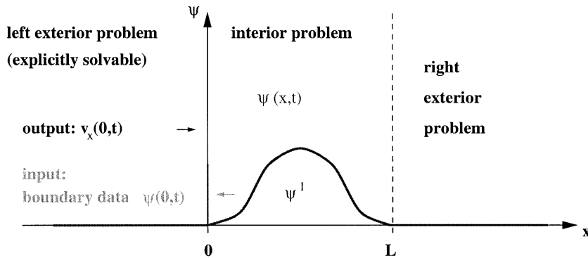
Fig. 1 - Schrödinger equation: Construction idea for transparent boundary conditions.
