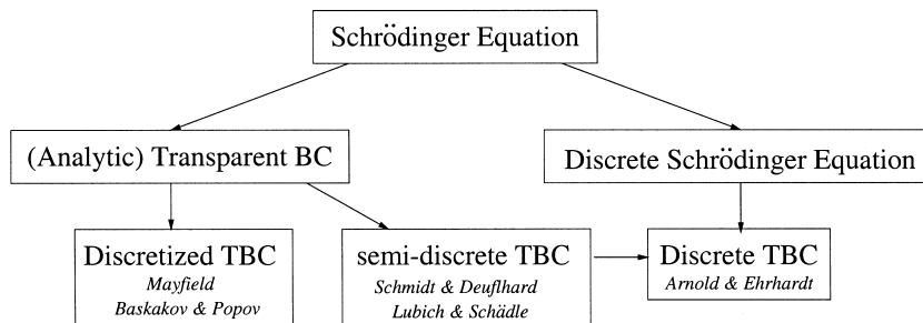
Fig. 3 - Discretization strategies for the TBC.
