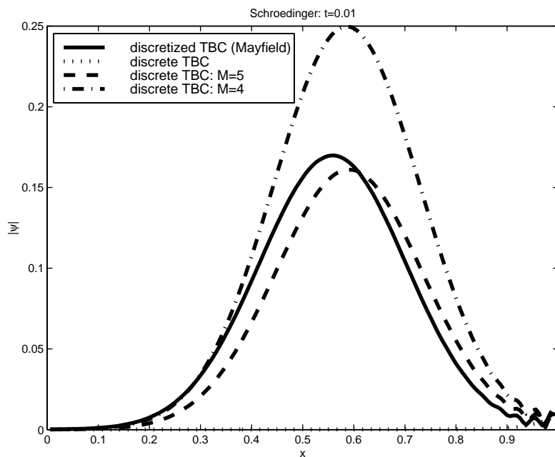
Fig. 7 - Solution |\psi(x, t)| at time t = 0.01 : the solution with the discretized TBCs of Mayfield [30] (—) in comparison to the solution using the simplified DTBC (3.85) with M = 4 (-.-.) and M = 5 (---).
